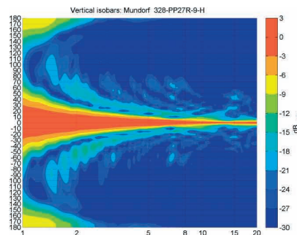
Vertical Dispersion 180°
