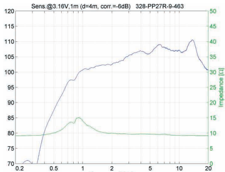
SPL 1W/1m - Impedance - Phase
