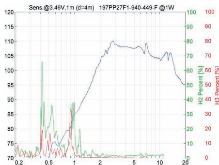
THD 1W
