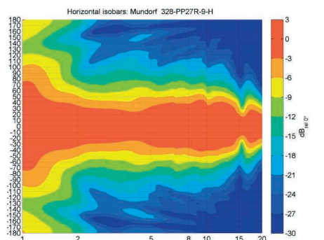
Horizontal Dispersion 90°
