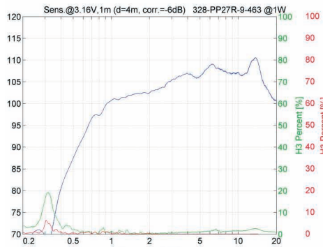
THD 1W
