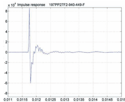
Impulsantwort / Impulse Response
