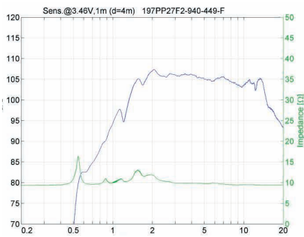
SPL 1W/1m - Impedance
