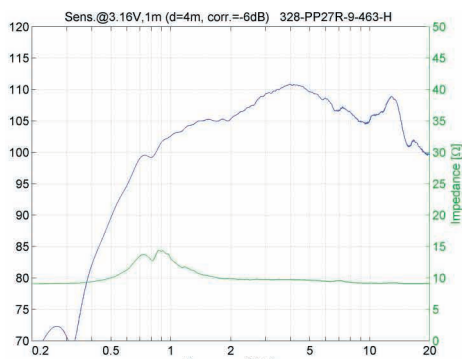
SPL 1W/1m - Impedance
